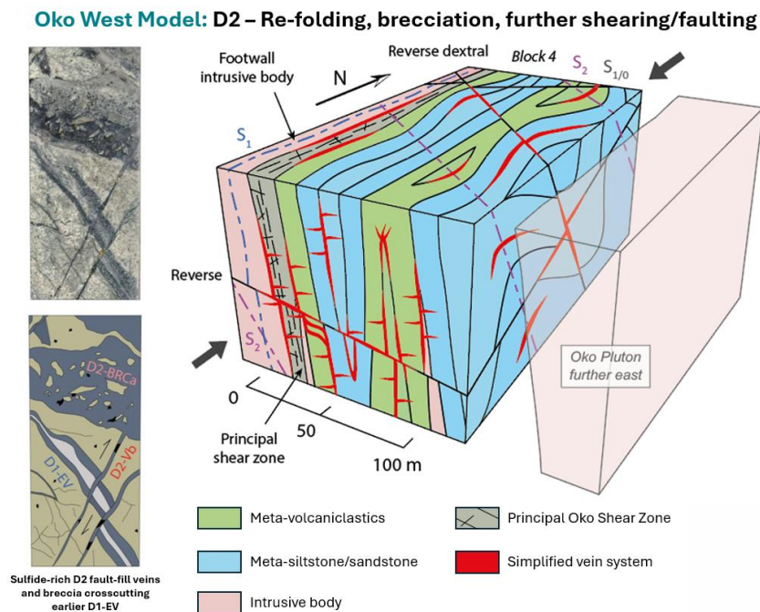
Figure 2: Oko West vein and polyphase deformation relationship model, excerpt from Hainque et al., 2025. 20
