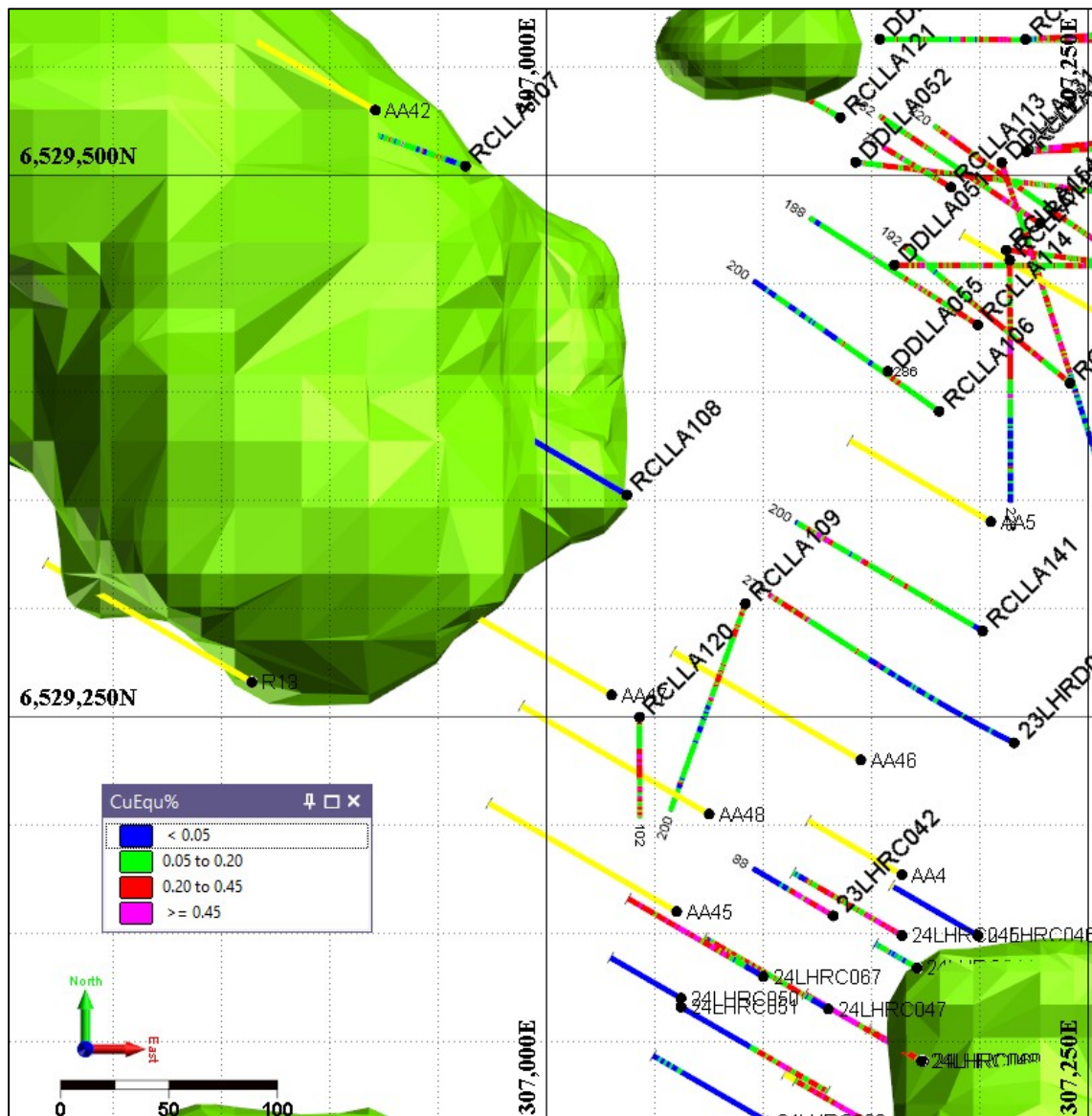
Figure 2 Location plan of planned drillhole AA48, note the large green shape is the new MT anomaly west of Ferro South at <50 ohm/ms.
