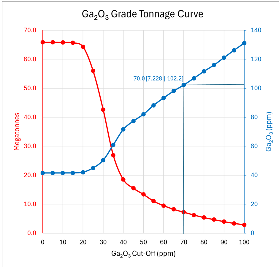
Figure 1 - Grade-Tonnage Curve
