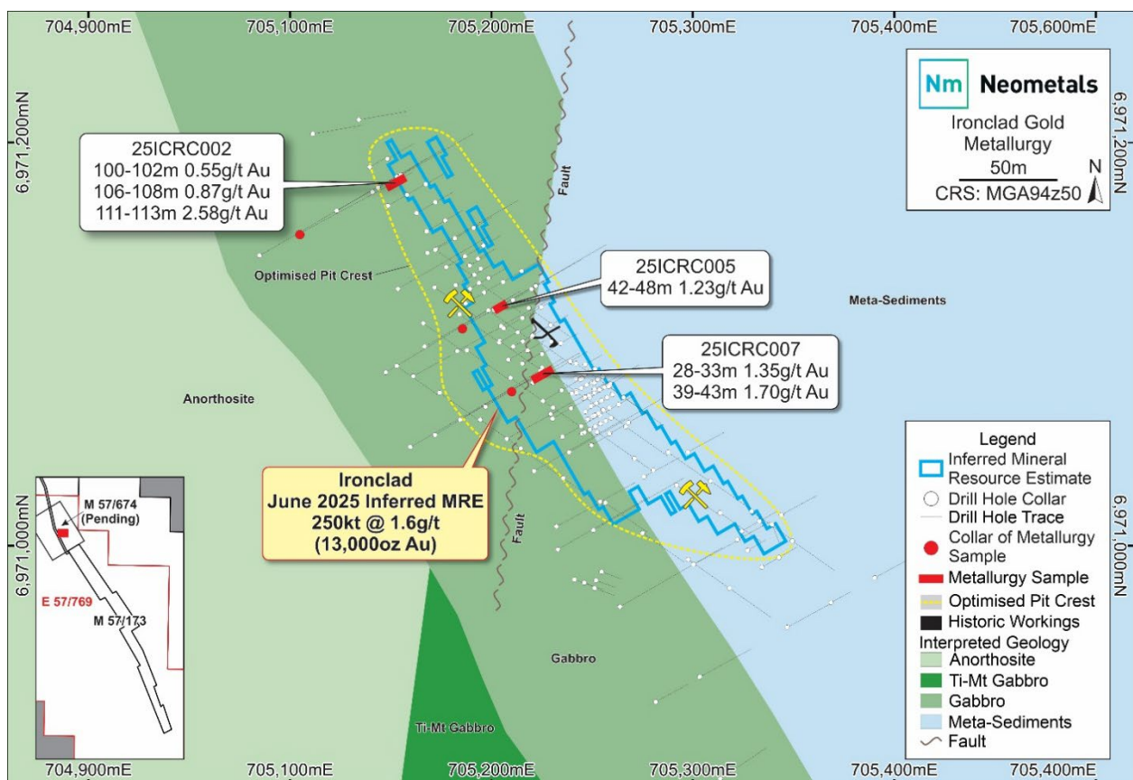
Figure 3: Plan showing location of RC holes 5 used for composites for Ironclad metallurgical test work. Also shown is an outline of the Ironclad Inferred MRE 2 and a representation of the optimised pit shell
