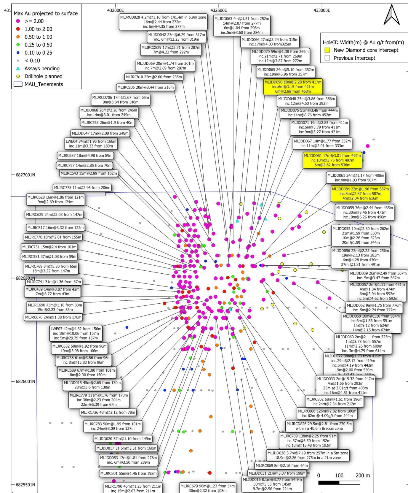
Figure 2. The Lady Julie North 4 deposit has numerous significant thick intersections from the latest drill programme (yellow large rectangular label) and previous drilling (white label) with maximum gold projected to surface and planned deeper drillholes (in yellow).
