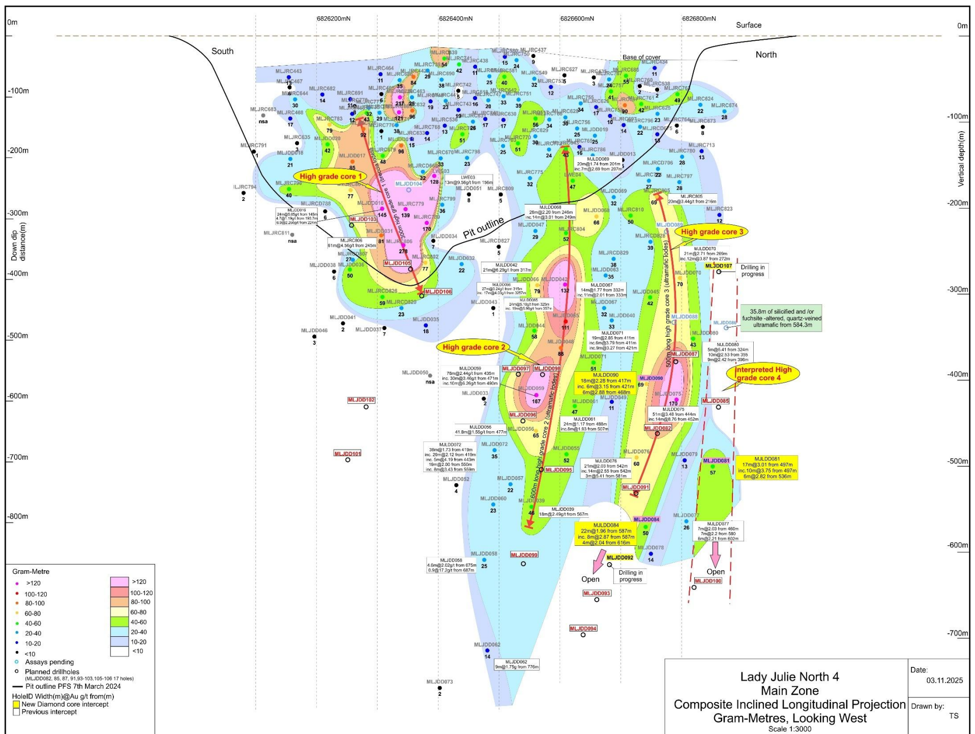
Figure 1. Composite Inclined longitudinal projection of the main lode in LJN4 in gram-metres. Highlighting continuous mineralisation over the whole 750m strike length. Three high grade core zones have been defined. The southern High-Grade Core Zone 1 is 300 x 200m in size and is associated with multiple silica pyrite and breccia lodes. High-grade Core zone 2 is 150m x 600m and is associated with altered silicified and fuchsite ultramafic lodes. The newly defined most northern high-grade core 3 is 150m x 500m and has similar alteration as core 2. Interpreted High-Grade Core 4 remains open at depth and up dip is currently being tested with further extension holes MLJDD085, MLJDD100 and MLJDD107.
