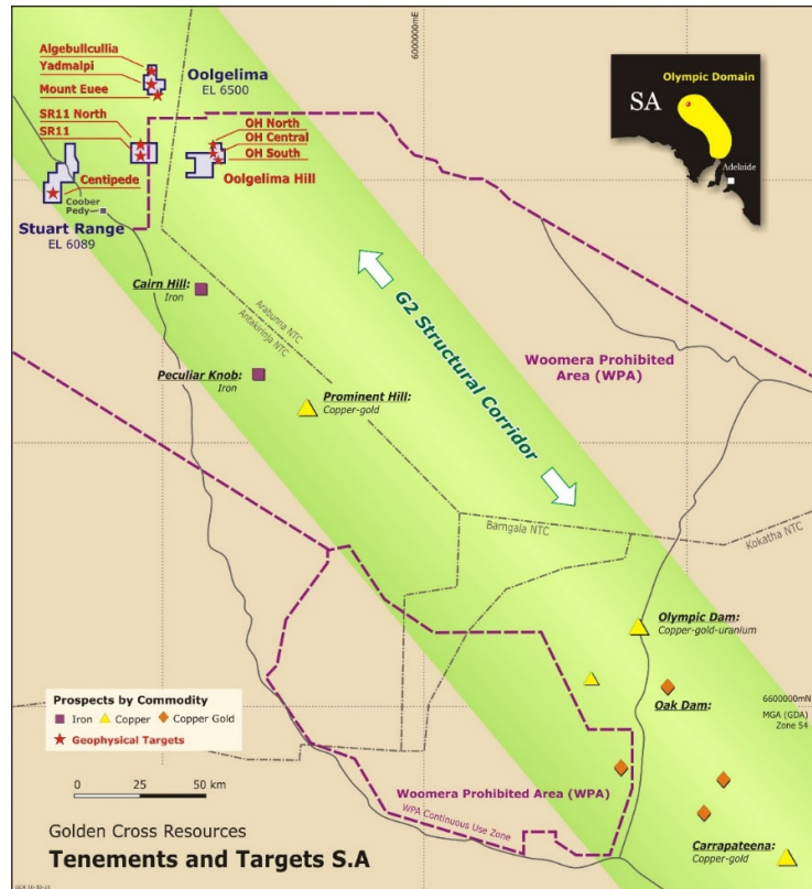
Figure 8: Gawler Craton Projects: Location & Drill Targets
