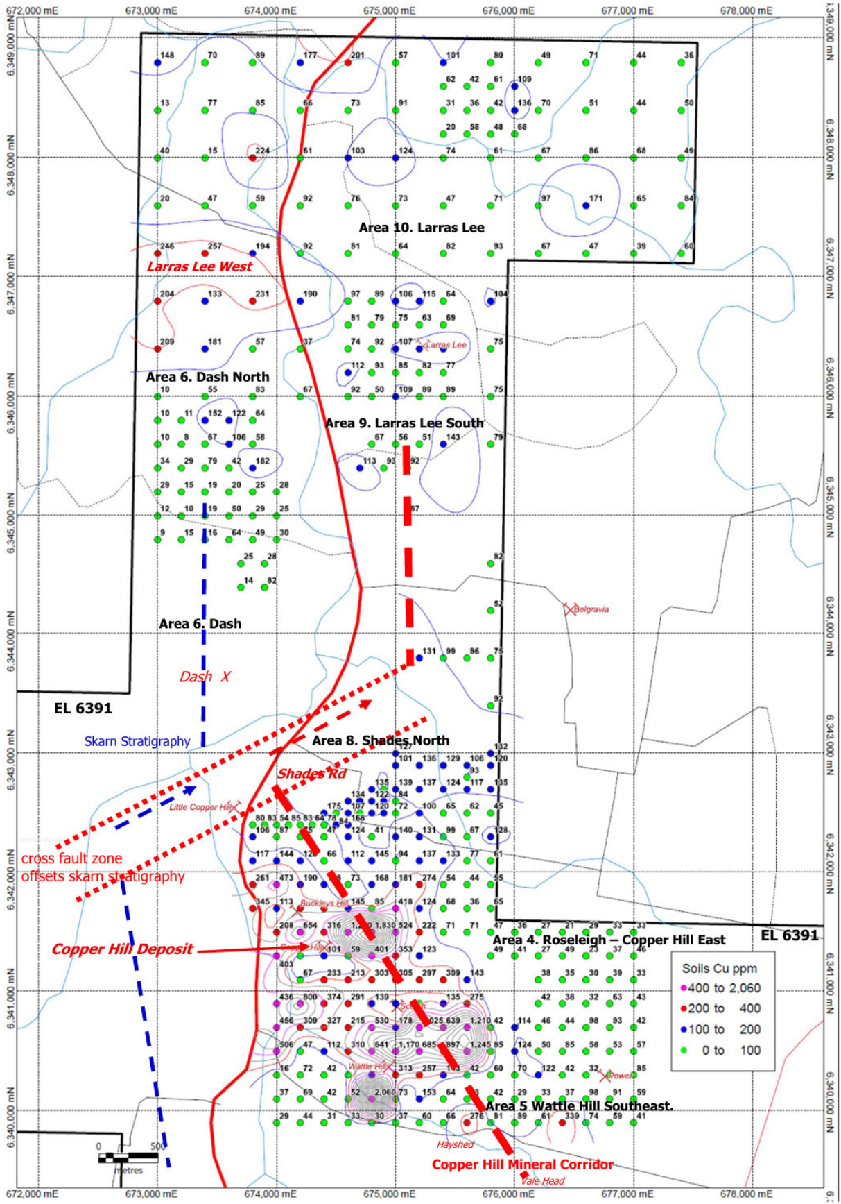
Figure 4: Geochemical Sampling areas – MGA Grid Northern EL6391 [Area 1-3 previously reported; Area 4 Roseleigh/Copper Hill East; Area 5 Wattle Hill Southeast; Area 6 Dash North; Area 7 Gamboola (see Figure 5); Area 8 Shades North; Area 9 Larras South; Area 10 Larras Lee;]
