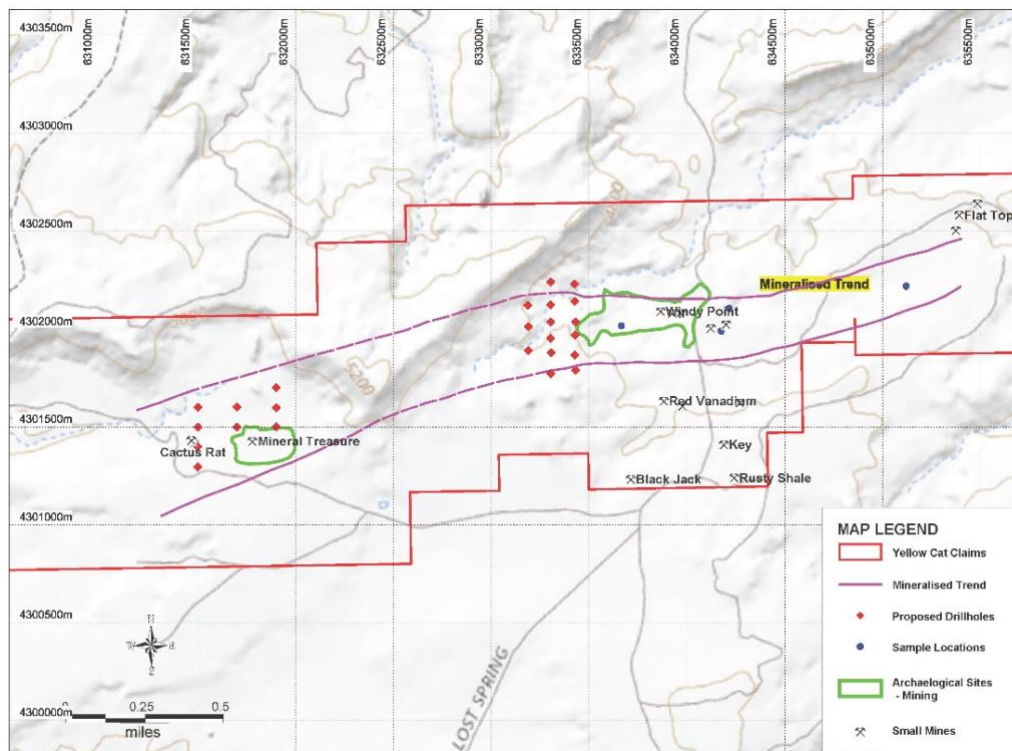
Figure 6: Plan showing the Yellow Cat planned drillhole locations and the U&V mineralization trend.
