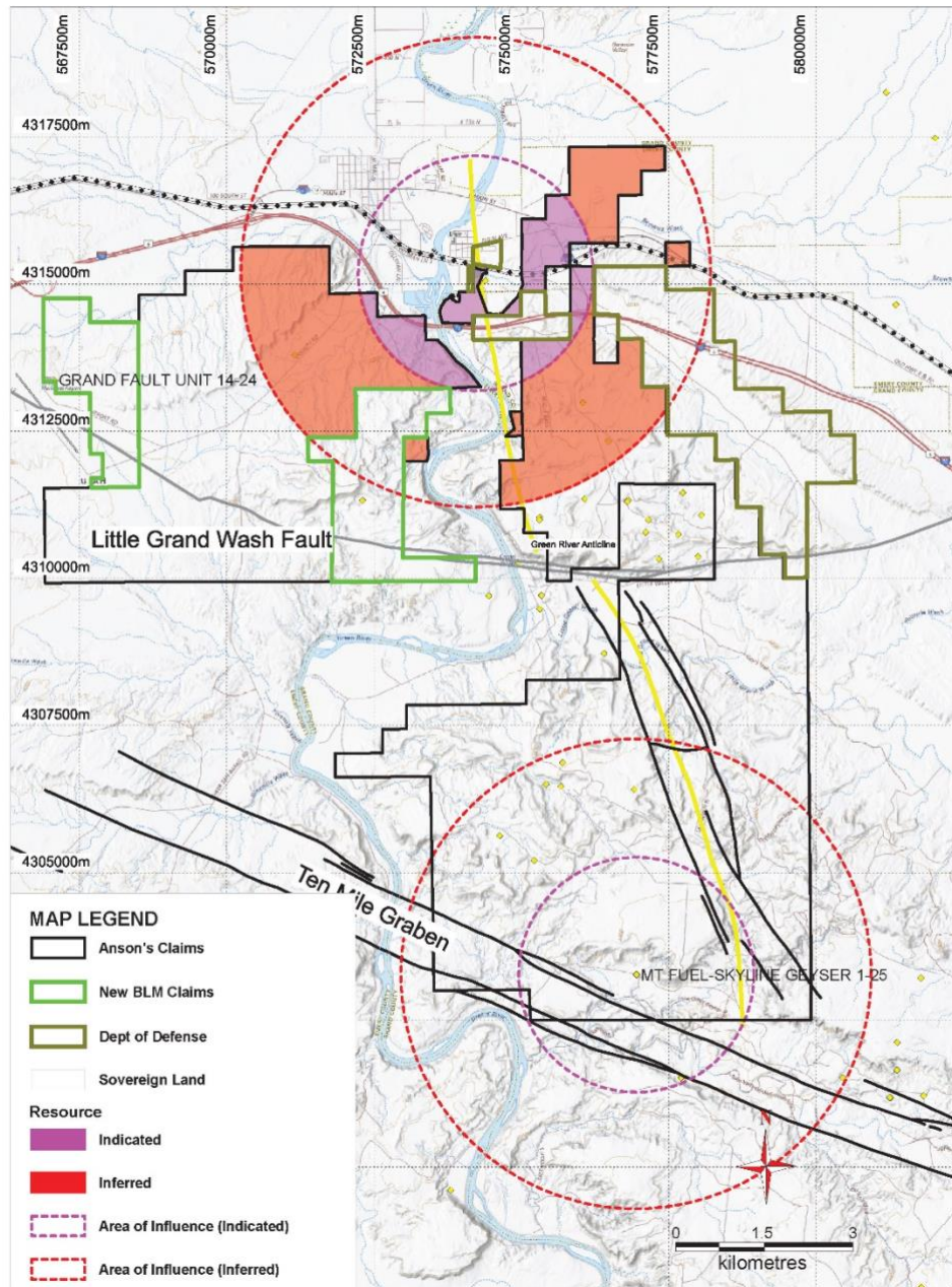
Figure 3: Plan showing the newly added claims in relation to the Maiden JORC Mineral Resource.
