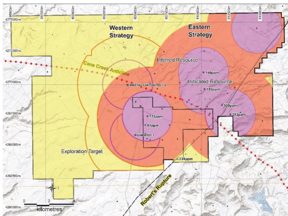
Figure 4: Plan showing proposed Areas of Influence (AOI) for the Western Strategy drilling program at Paradox Project.
