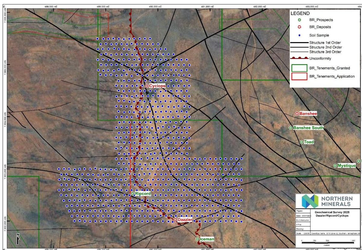
Figure 2: Soil sampling (UFF+) locations covering unconformity from Dazzler to Cyclops.
