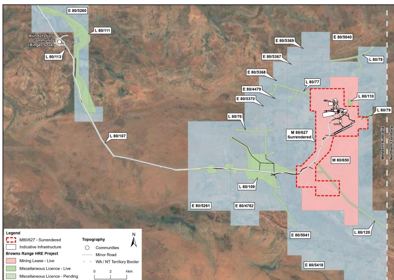
Figure 1: Map of Browns Range project tenure.
