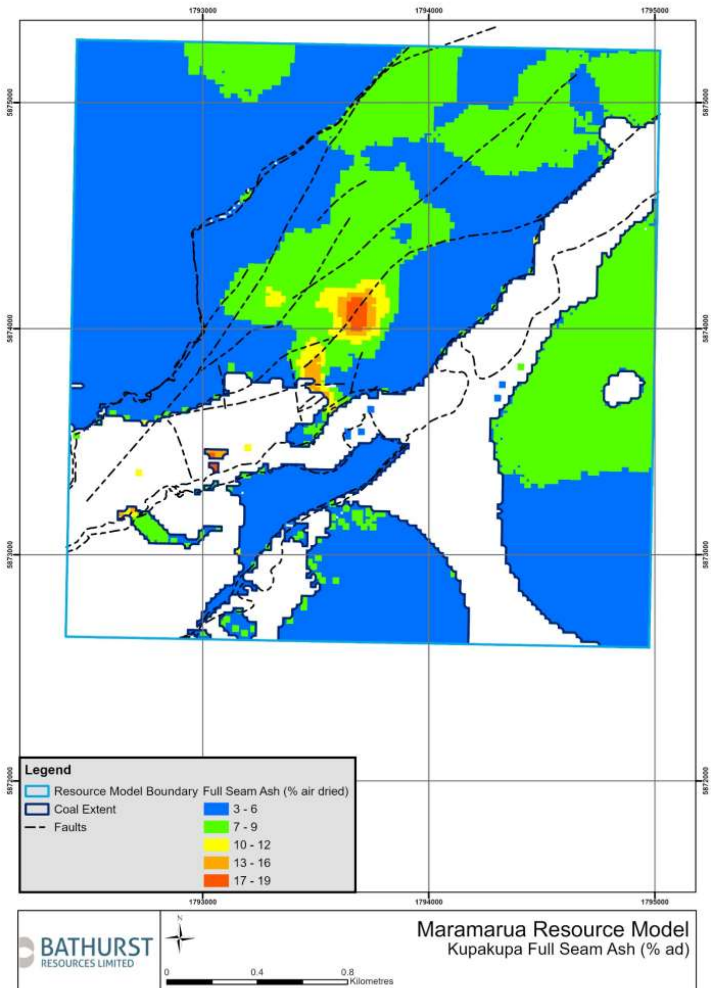
Figure 10: Plan showing in situ full seam ash distribution of the Kupakupa coal seam
