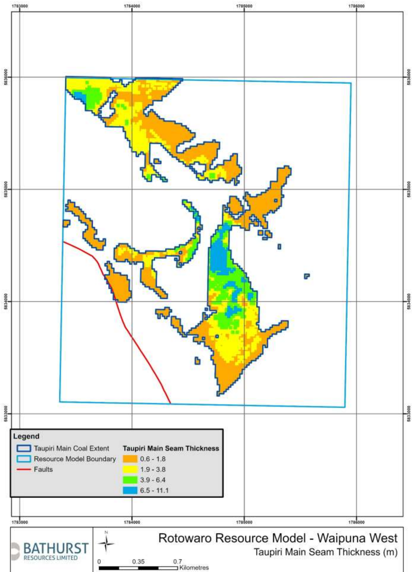
Figure 10: Plan showing Taupiri seam thickness distribution over the Waipuna West resource area
