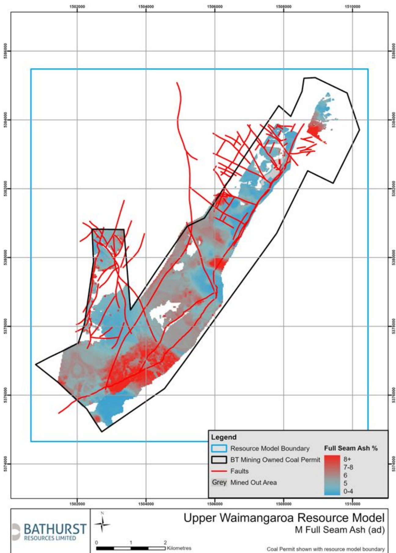
Figure 12: Plan showing in-situ full M seam ash on an air dried basis across the Upper Waimangaroa South resource
