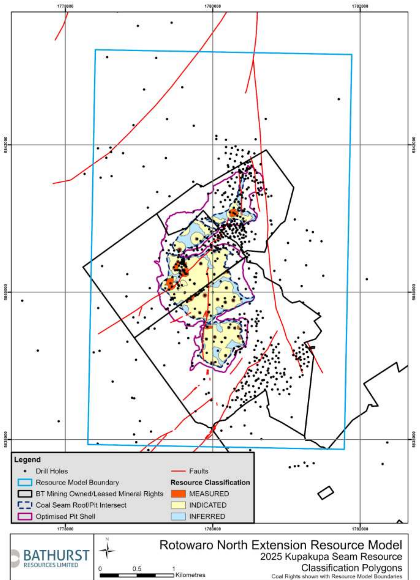
Figure 7: Plan showing the resource classification polygons for the KK seam
