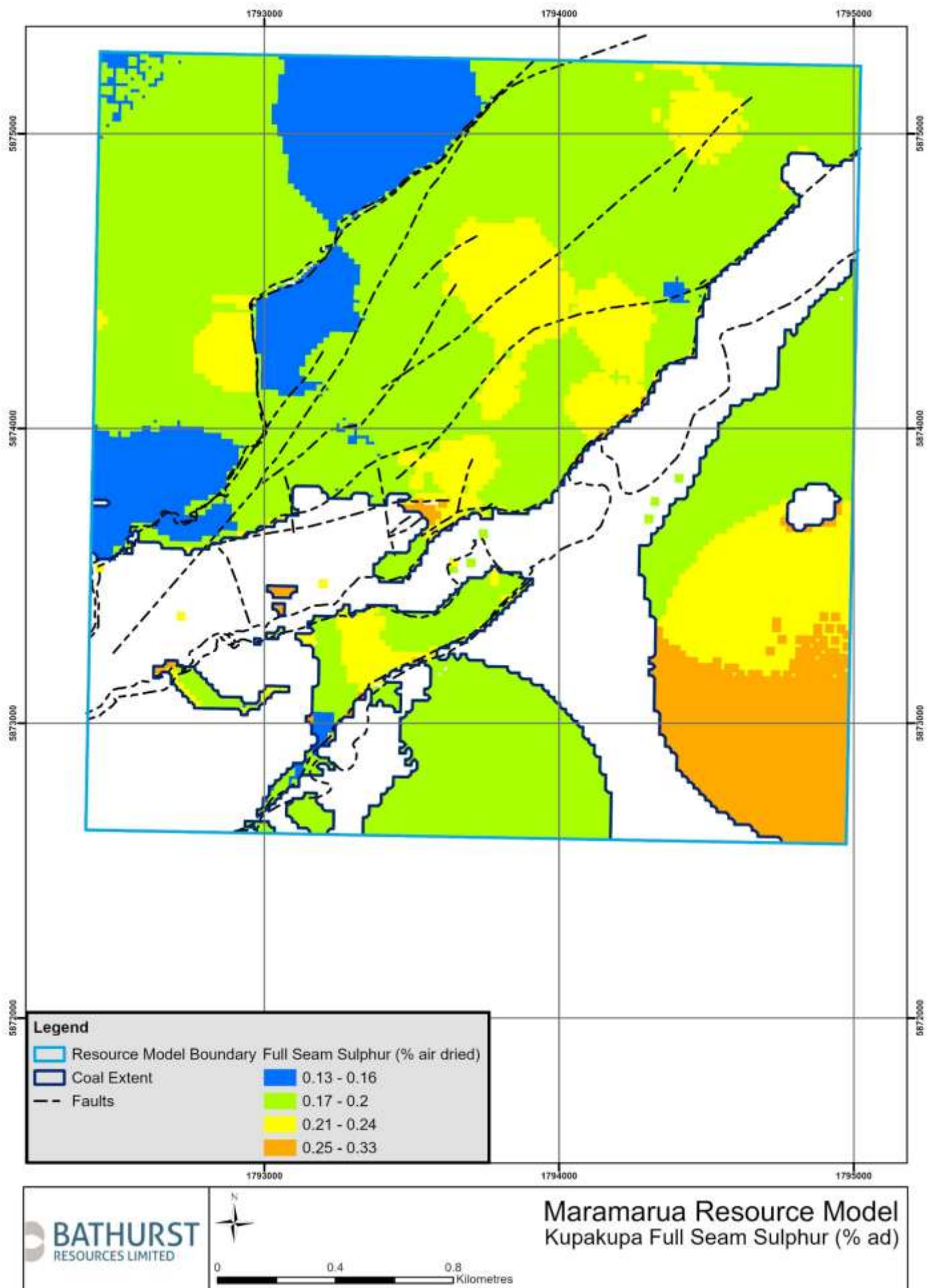
Figure 11: Plan showing full seam sulphur distribution of the Kupakupa coal seam
