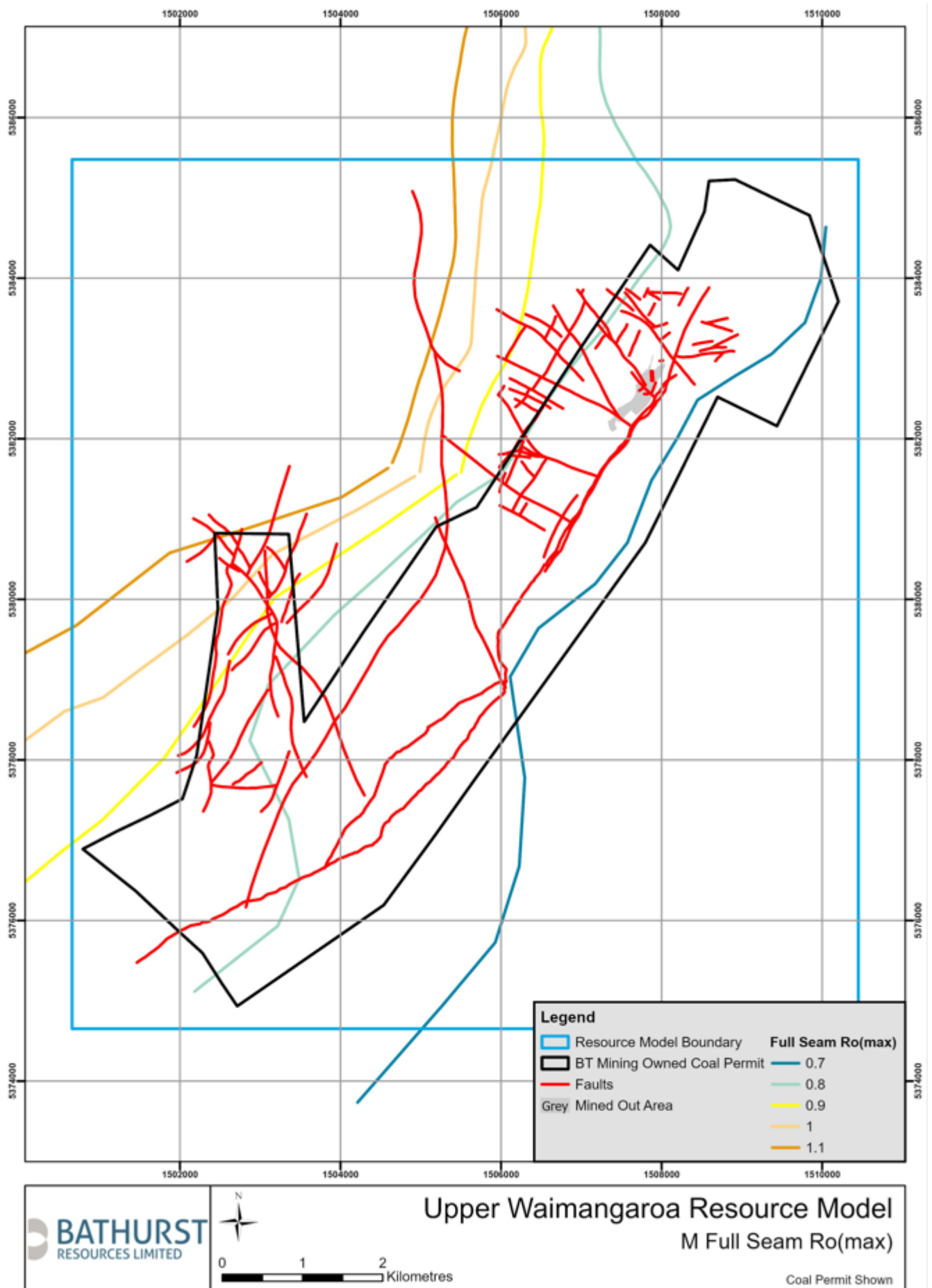
Figure 16: Plan showing the Romax for the M Coal Seam
