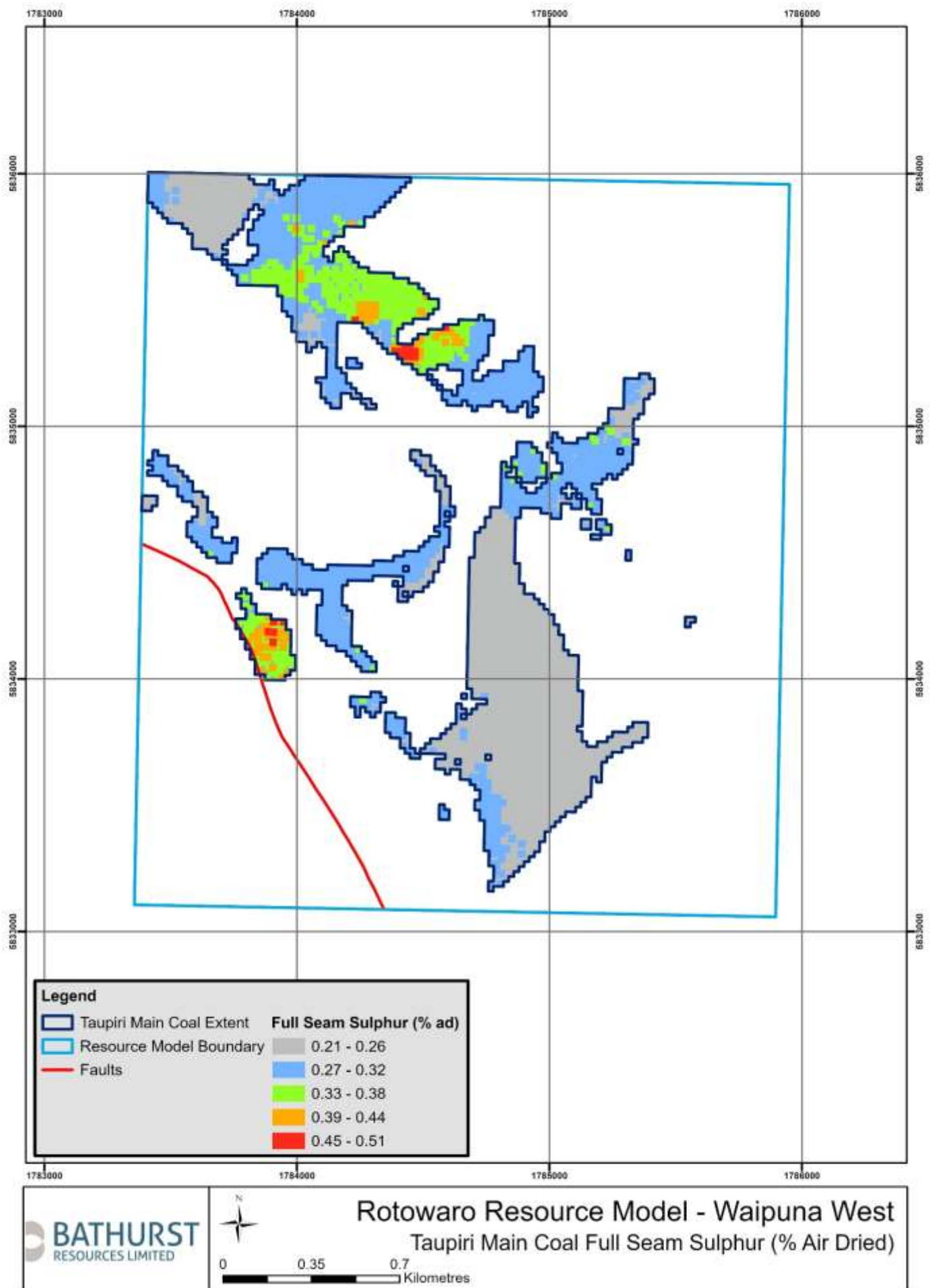
Figure 12: Plan showing Taupiri seam sulphur on an air-dried basis distribution over the Waipuna West resource area
