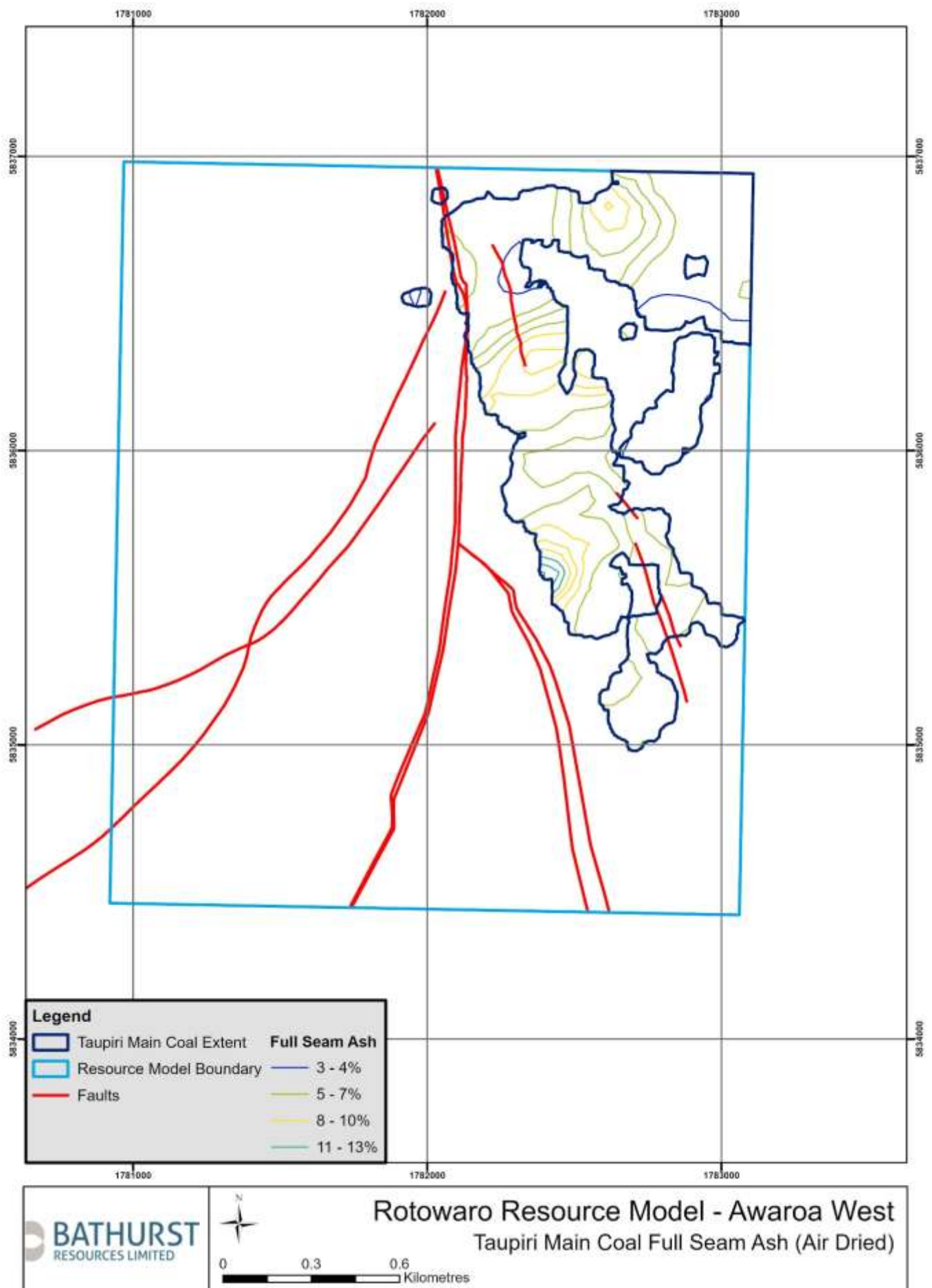
Figure 2144: Plan showing in situ Taupiri seam ash on an air-dried basis as modelled over the Awaroa West resource area
