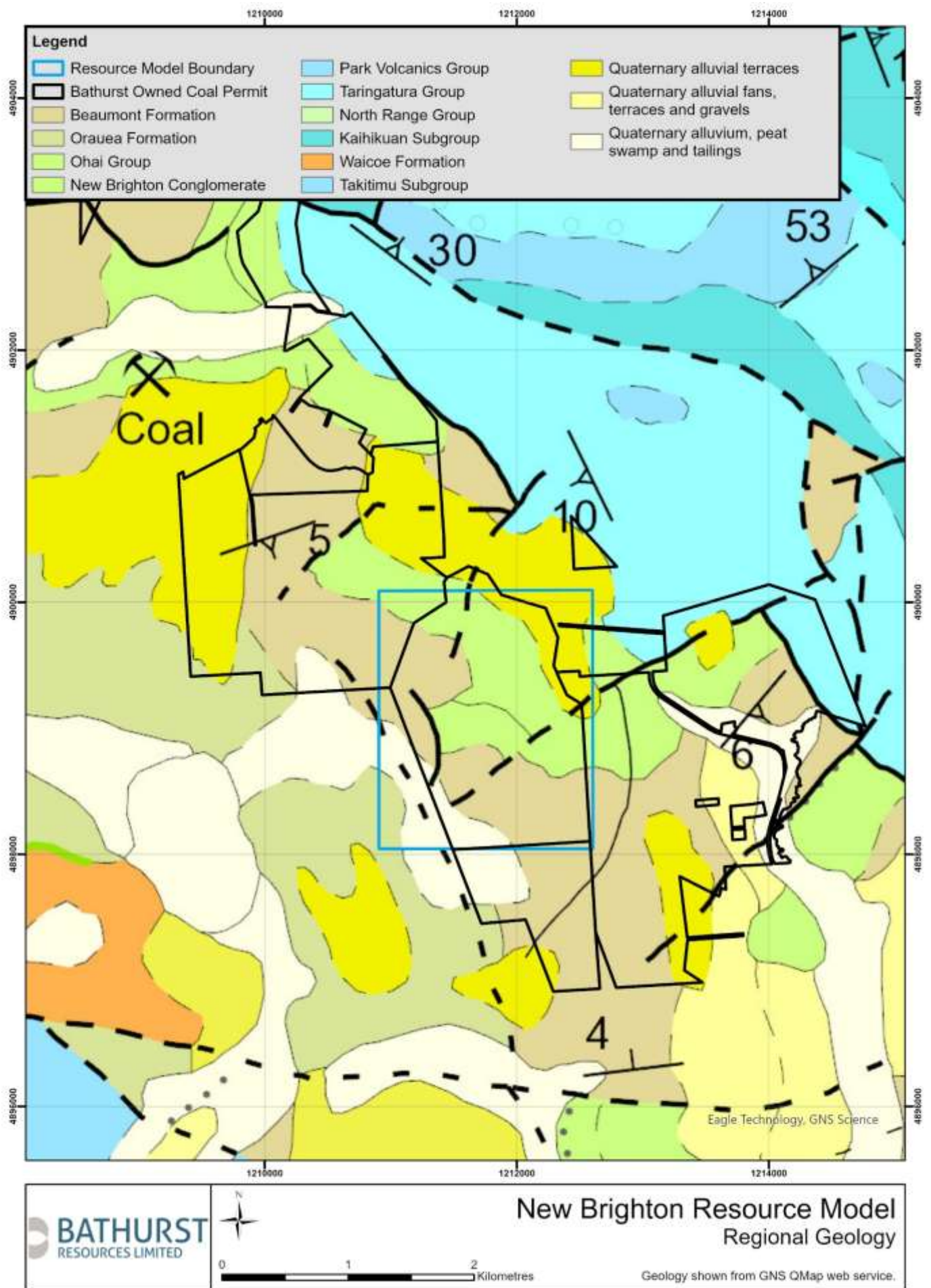
Figure 2: Regional Geology
