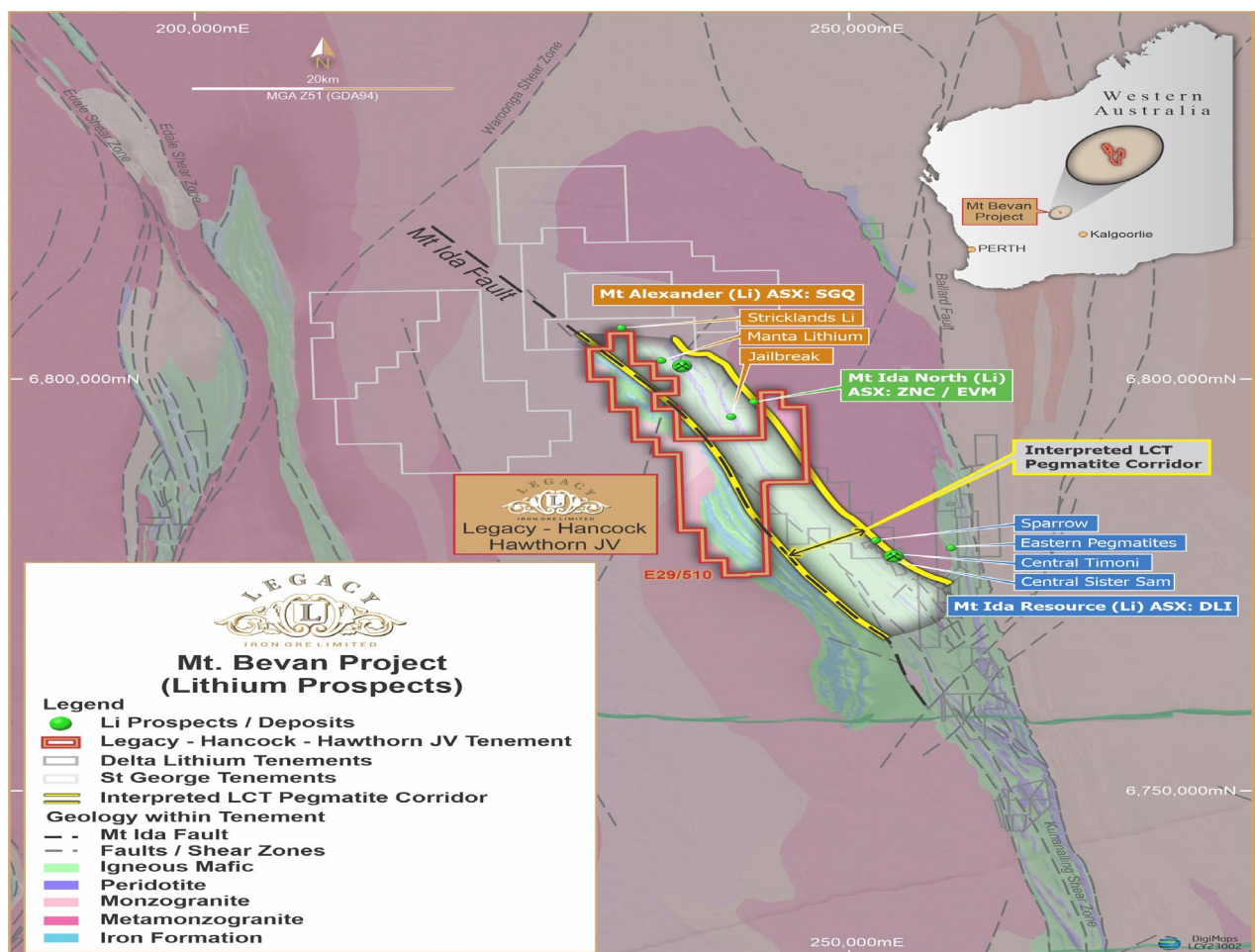
Figure 30 Mount Bevan Project, LCT pegmatite corridor
