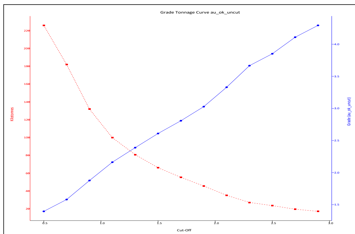
Figure 14 Grade tonnage curve for Golden Rainbow
