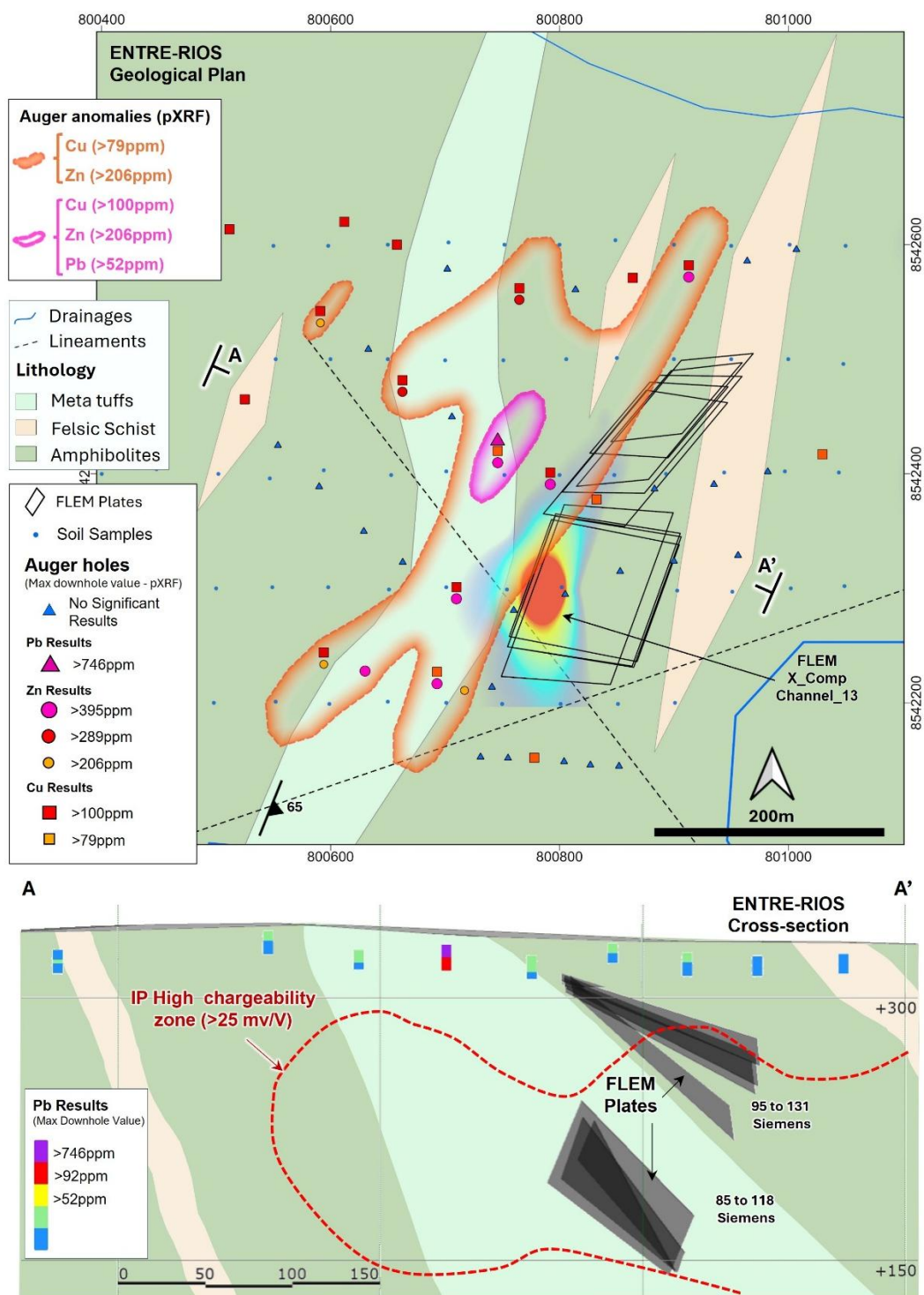
Figure 5: Entre Rios Prospect, geological plan and section.
